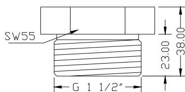
G 1 1/2" A TM 7
