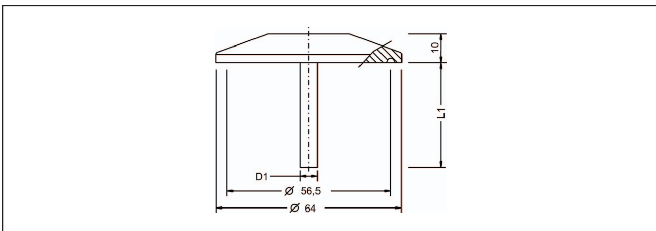
Type T - Clamp ISO 2852 DN51 (2") / DIN 32676 DN50
