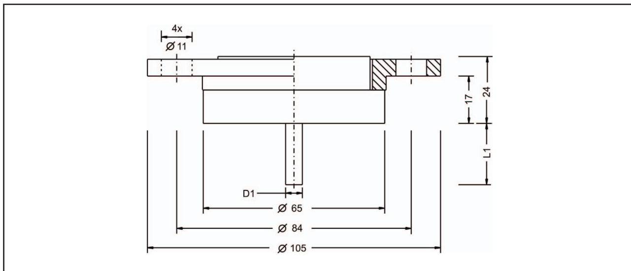
Type L - DRD DN50, Ø65 mm
