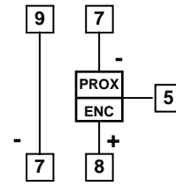
INPUT FOR PROXIMITI AND ENCODER AMPLIFIED 24 VDC
