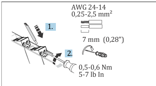
1 Electrical connection
