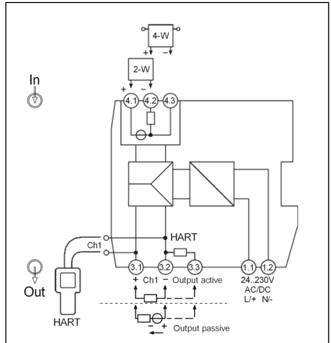
2 Terminal assignment
