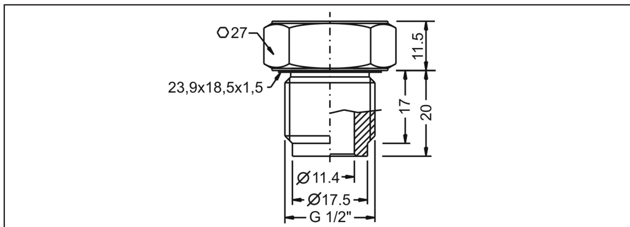
Type 2 – Thread ISO 228-1 – G½"B, inner bore
