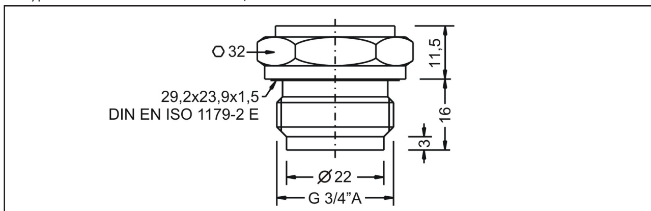
Type 8 – Thread ISO 228-1 – G¾"A, front-flush
